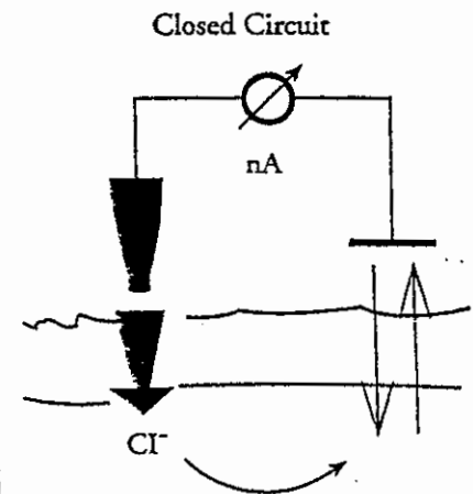
Figure 1: Schematic representation of current measurement without use of an external voltage source. A pointed electrode placed on an acupuncture point taps the current, which may develop as a result of the conductivity of chlorides. A reference electrode with a large surface area rests on the subject's forearm.
